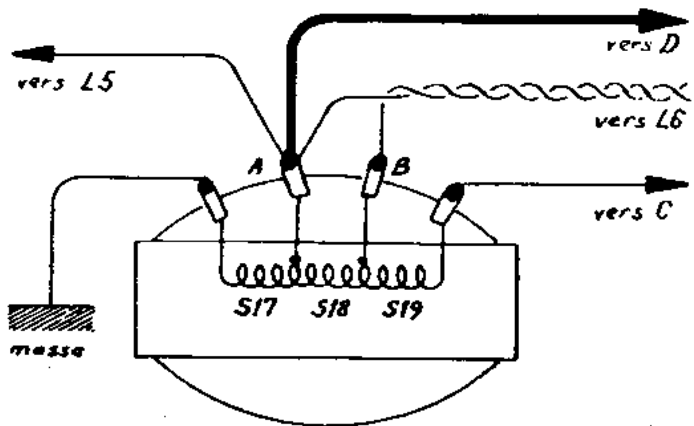
Branchement 117 V.
