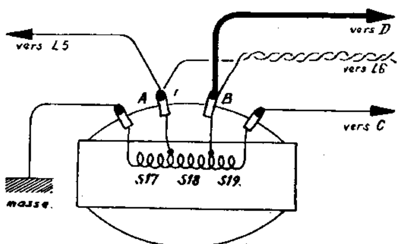
Branchement 123 V.
